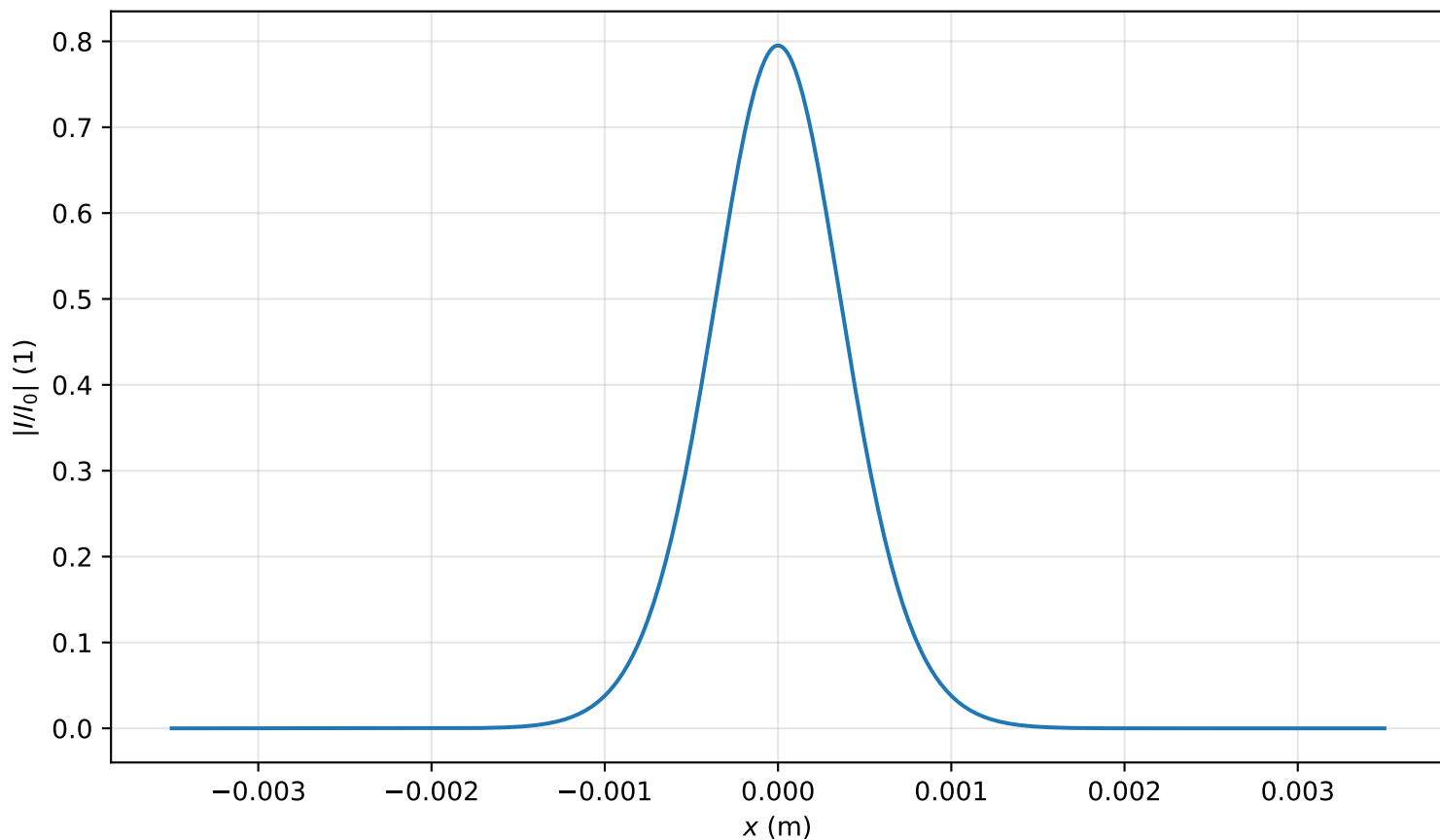
Intensity profile I(x, y = 0, z = 1.513m)/I_0 , P_{in}=0.3P_{cr} , artificial time
